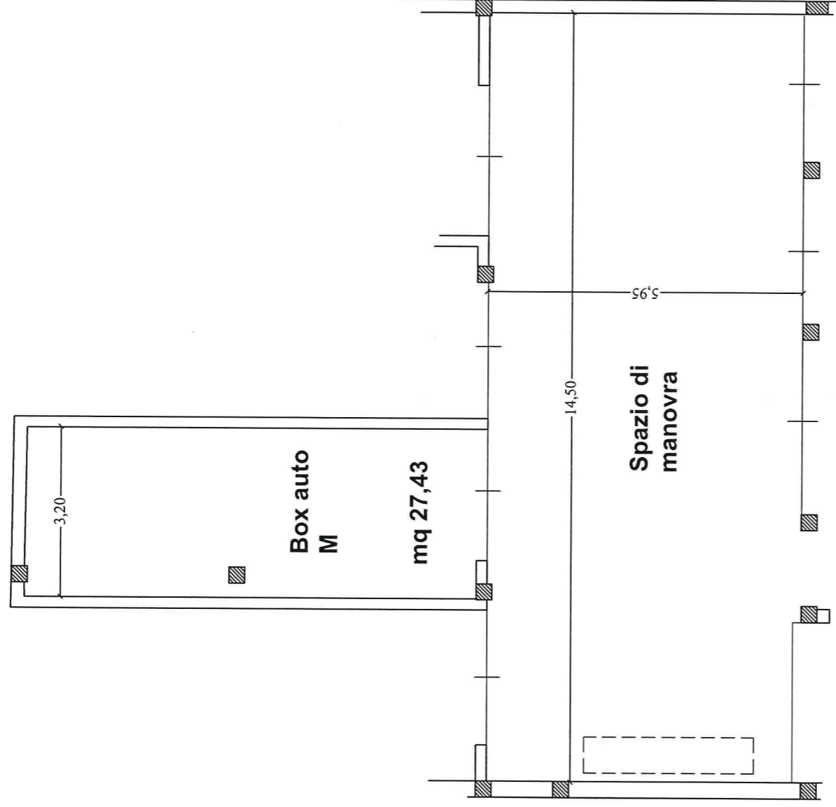
PIANO INTERRATO
